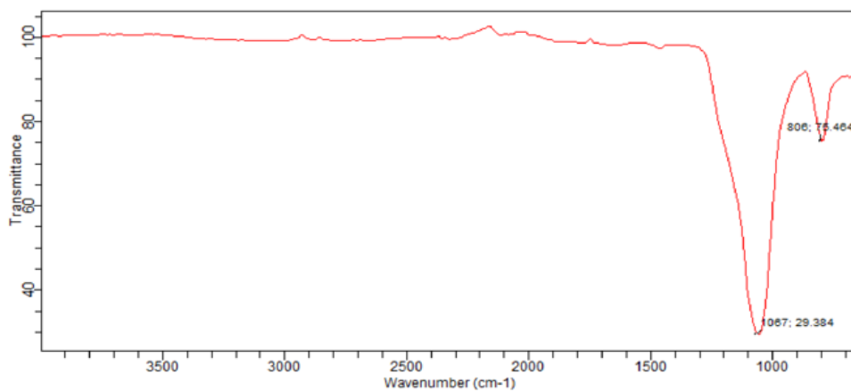
Figure 3.2 Spectrum of FT-IR Silica with Glycerol Template
