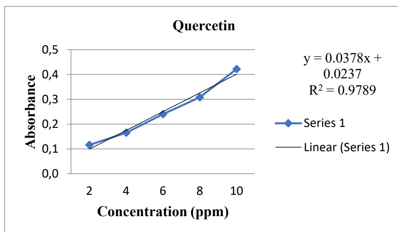
Figure 5. Quercetin standard solution curve
