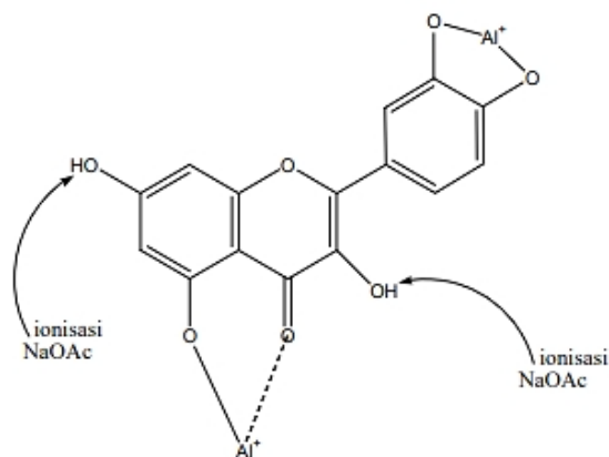
Figure 4. The reaction between flavonoid groups with \text{AlCl}_3 forms a stable acid complex[34].
