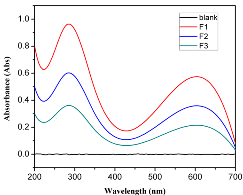
Figure 3. UV Vis Spectrum of Coffee Grounds Extract
