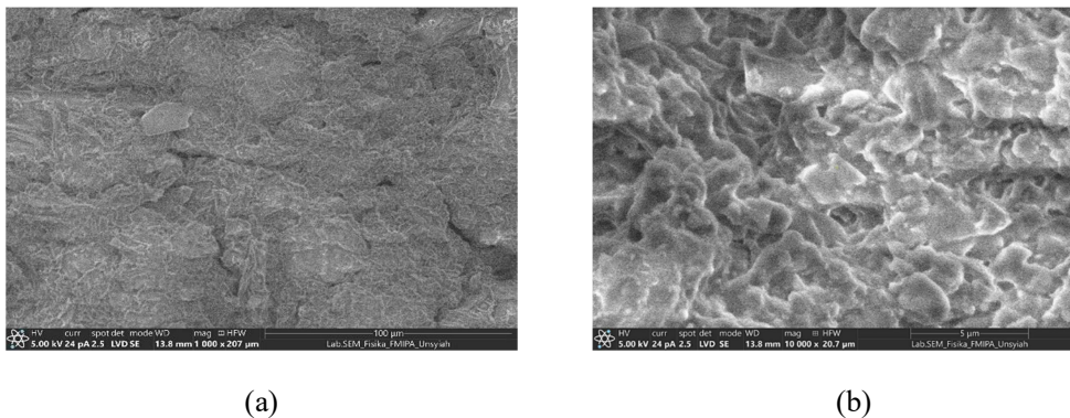
Figure 8. (a) SEM-EDX test of sample B (5:20:25) 1000 \times magnification, and (b) SEM-EDX test of sample B (5:20:25) 10000 \times magnification.
