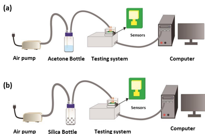
Figure 1. Illustration of sensor testing against (a) acetone gas and (b) sensor recovery with silica gel.
