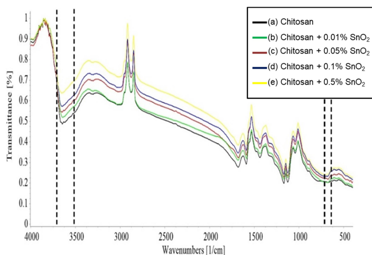
Figure 4. FTIR characterization results of (a) chitosan film, (b) chitosan-0.01% \text{SnO}_2 , (c) chitosan-0.05% \text{SnO}_2 , (d) chitosan-0.1% \text{SnO}_2 , and (e) chitosan-0.5% \text{SnO}_2 .
