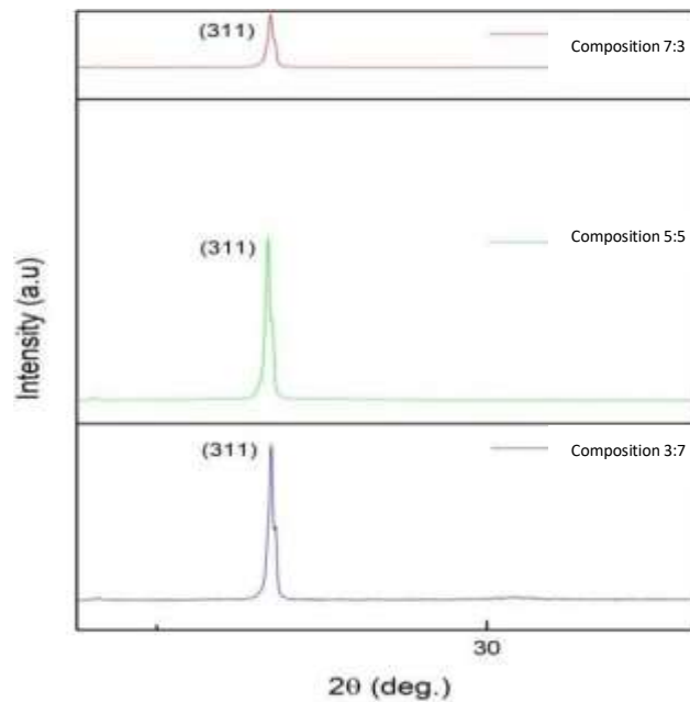
Figure 2. The enlarged peak of 311 of all compositions
