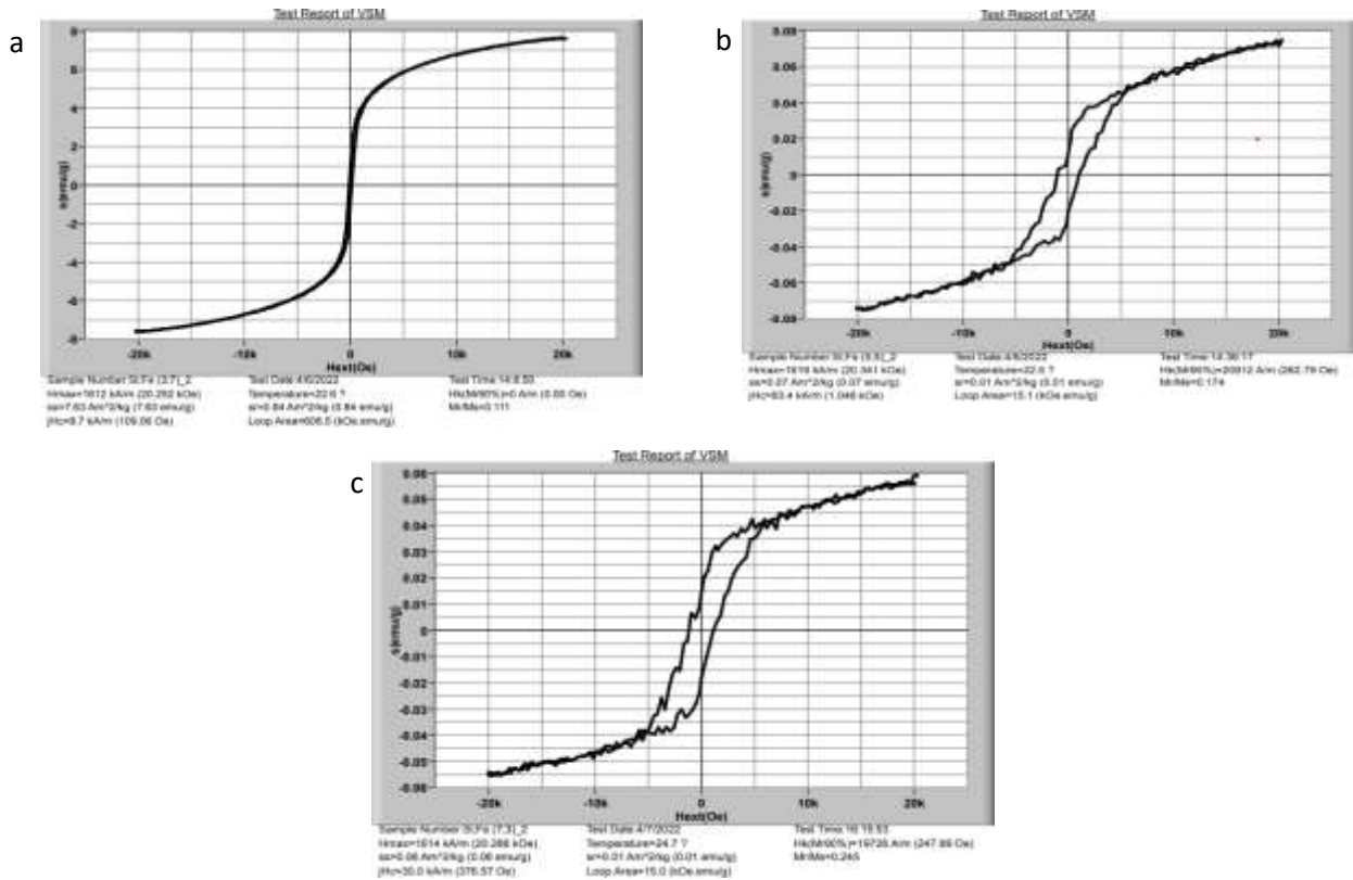
Figure 6. The hysteresis curve of (a) sample 1 on \text{SiO}_2\text{-Fe}_3\text{O}_4 (Composition 3:7); (b) sample 2 on \text{SiO}_2\text{-Fe}_3\text{O}_4 (Composition 3:5); (c) sample 3 on \text{SiO}_2\text{-Fe}_3\text{O}_4 (Composition 7:3)
