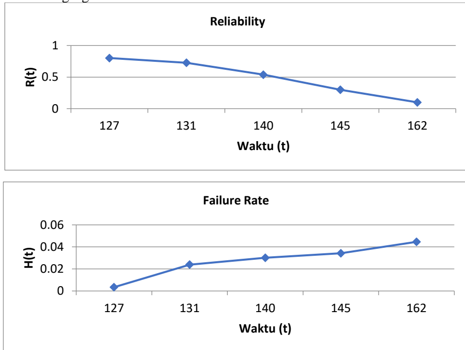
Figure 5. Reliability and Failure rate graphics Link wheel
