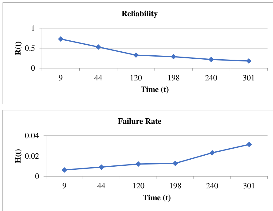
Figure 4. Reliability and Failure rate graphics return rail
