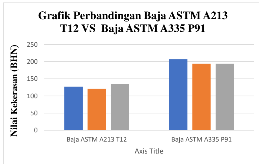
Figure 5. Graph Comparison of hardness
