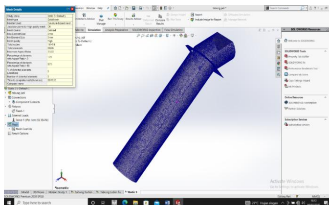
Figure 7. Meshing Process.
