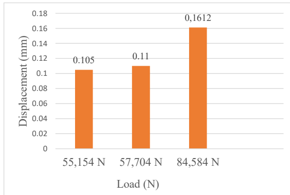
Figure 21. Displacement Graph with Load Variation
