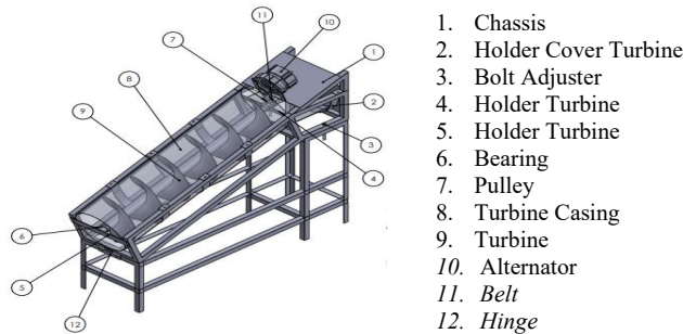
Figure 3. Design of Archimedes Screw Turbine.
