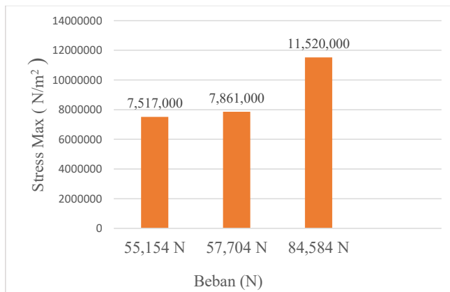
Figure 11. Graph of Maximum Stress versus Load Variation
