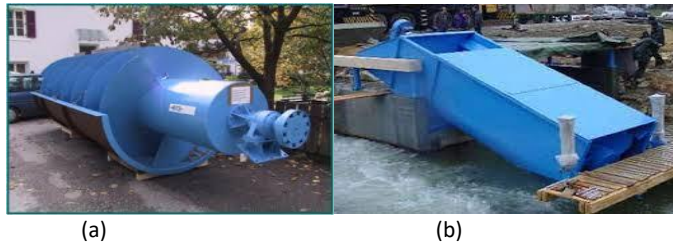
Figure 2. Screw Turbine: (a) Steel Trough Type and (b) Closed Compact Installation Type
