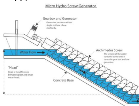
Figure 1. Schematic AST Turbine [10]
