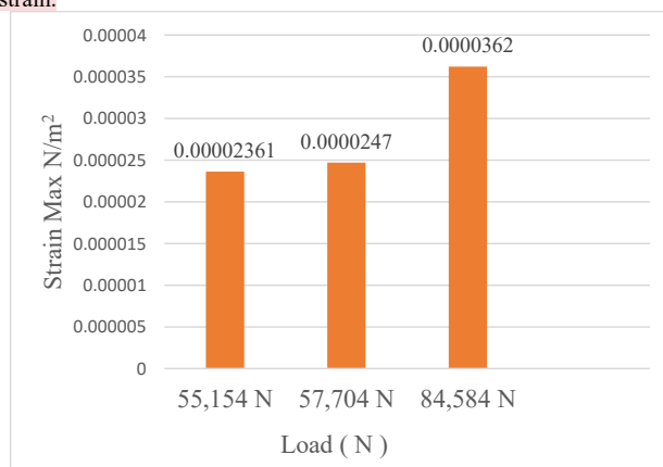
Figure 16. Maximum Strain Graph with Load Variation
