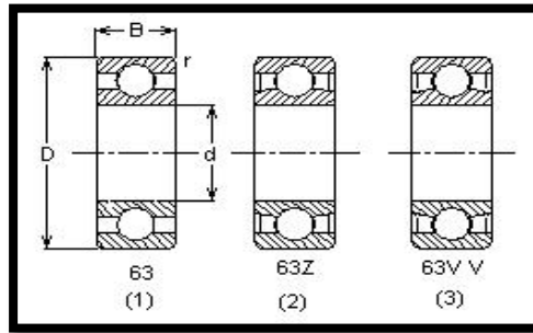
Gambar 4. Bantalan [4]
