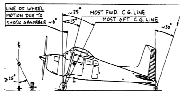
Gambar 2.1 Landing Gear
