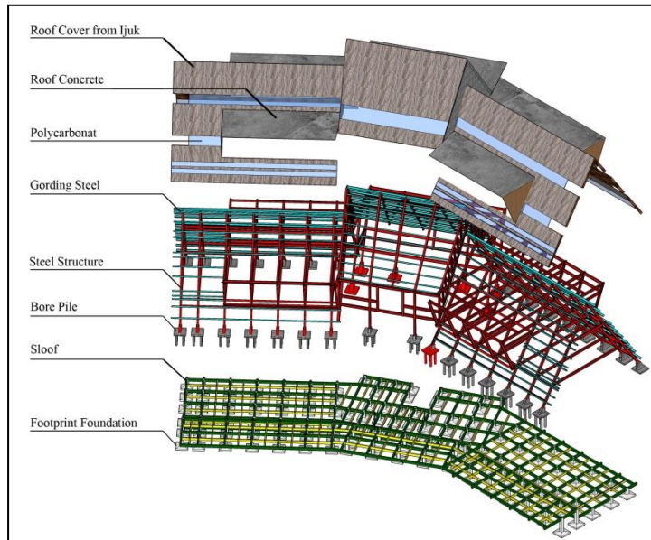
Figure 7. Axonometry of structure
