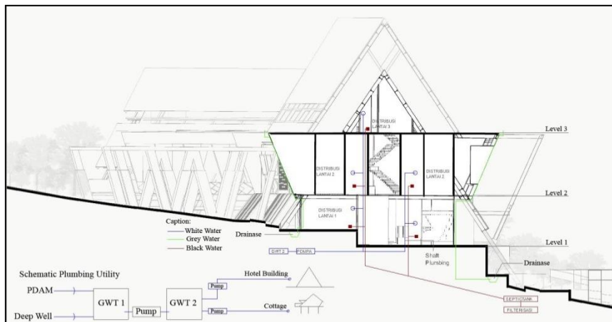
Figure 10. Schematic Plumbing utility
