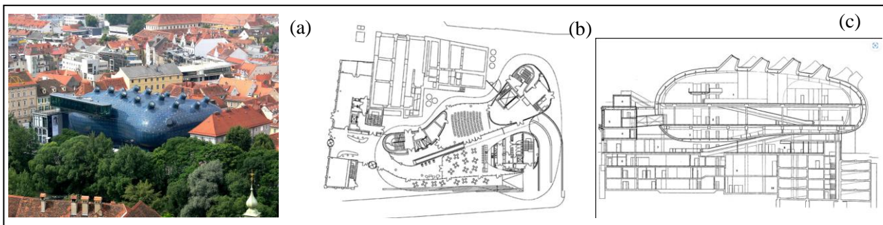
Figure 1 (a) Original Condition of The Kunsthau Graz; (b) Site plan; (c) Section
