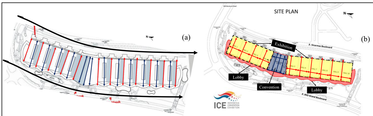
Figure 8 Dimensions in ICE BSD Building (a) Dimensions on the exterior; (b) Dimensions on the interior
