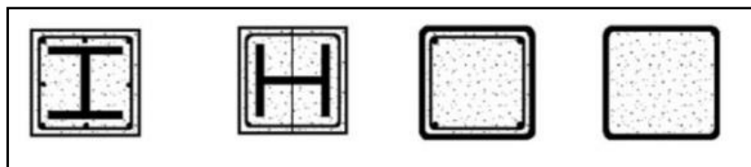
Figure 11. Composite Steel Column (Source: [2] Hindarto, 2012)
