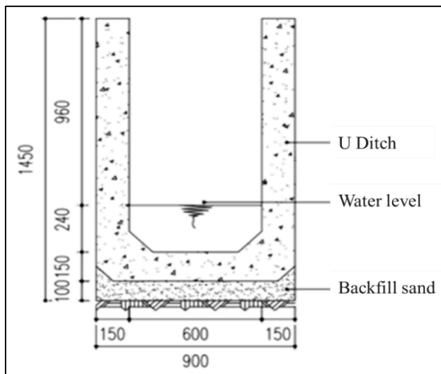
Figure 2 Drainage Section at Tuamang Road
