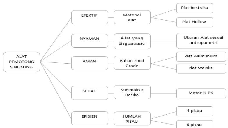
Gambar 2. Objective Tree
