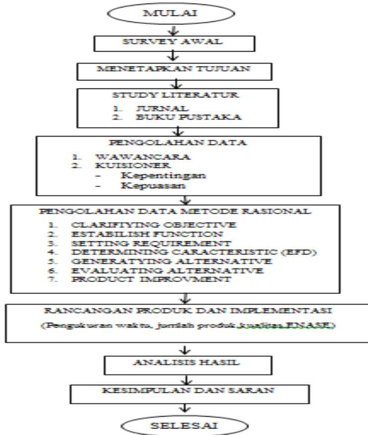
Gambar 1. Alur penelitian
