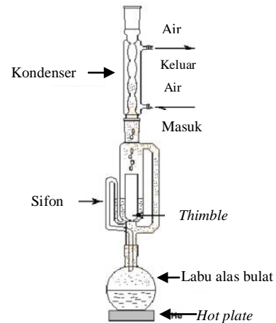
Gambar 1. Peralatan Sokhlet
